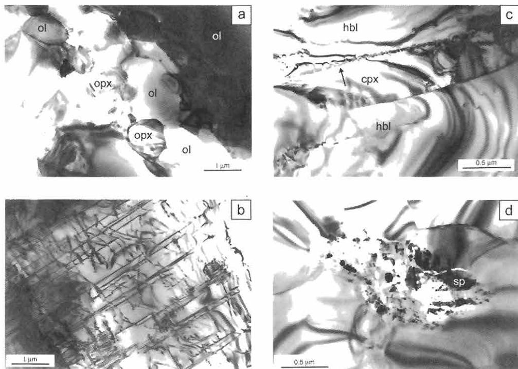
Fig. 7. Transmission electron microscope (TEM) images of mylonite in type 1 shear zone. (a) Olivine and opx grains in mixed phase laminae derived from spinel and cpx porphyroclasts. The very fine grains are dislocation-free and have equant shapes. (b) Dislocations within an olivine grain from a dynamically recrystallized monophase olivine layer (average diameter 20–50 \mu\text{m} ) in the tail of an olivine porphyroclast. Note the well-organized subgrain walls. (c) View parallel to the c -axis of a clinopyroxene grain (oriented east-west in center) between two pargasitic hornblende grains. The upper boundary of the cpx grain (arrow) is coherent along the shared a and b crystallographic directions of cpx and hornblende. Mottled contrast along this boundary reflects steps in the coherent boundary. (d) Pseudomorphous replacement of spinel (sp) by an aggregate of serpentine, chlorite and magnetite. Small spinel aggregates are found in some of the pseudomorphous aggregates.
