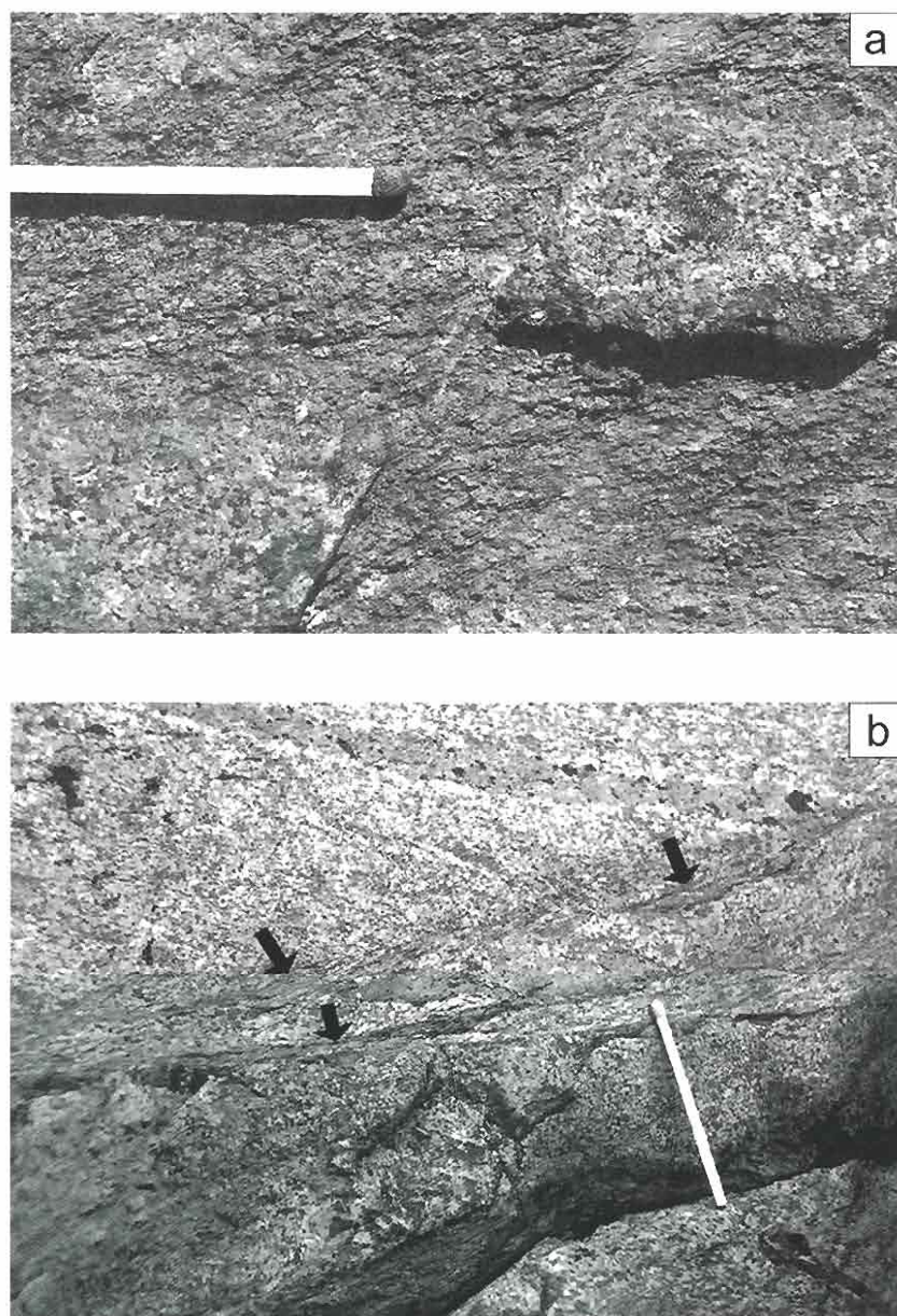
Fig. 4. Type 1 shear zones. (a) Shear zone offsets cumulate pyroxenite layer. Match for scale is 5 cm long. (b) Shear zones defined by closely spaced mylonitic foliation (arrows) truncates granulite facies schistosity and is related to vein-type pseudotachylite (above match tip).
