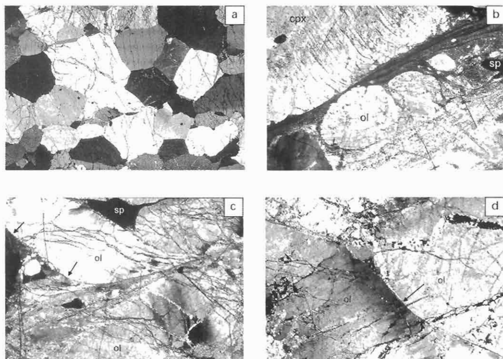
Fig. 5. Microstructures of a type I shear zone and its host rock, as observed in a polarizing light microscope with crossed nichols in the XZ fabric plane. (a) Protogranular microstructure of the host spinel lherzolite (frame length = 11.5 mm). (b) Thin mylonitic band at edge of shear zone in Fig. 4a. Note truncated twins in clinopyroxene (cpx), rounded clasts of olivine (ol), and spinel (sp) in ultrafine grained matrix of olivine, plagioclase, and hornblende (frame length = 1.35 mm). (c) Mylonitic microstructure in shear zone depicted in Fig. 4a. Arrows point to one of several arcuate cracks emanating from the side of the shear zone (frame length = 3.4 mm). (d) Close up of tip of crack in olivine grain indicated by arrows in (c). (frame length = 1.35 mm). Note undulose extinction adjacent to the crack.
