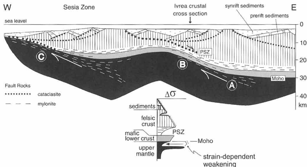
Fig. 11. Schematic cross section through the Apulian margin of Tethys at the end of Early Mesozoic rifting (after Handy & Zingg 1991; Schmid 1993). A, location for nucleation of type 1 shear zones; B, location for activity of type 2 shear zones; C, trans-lithospheric shear zone exhuming subcontinental mantle to the ocean floor. Approximate location of present Sesia Zone is labelled. Geometry of rift basins adopted from the references above. PSZ, Pogallo Shear Zone, as in Fig. 1a. Strength versus depth diagram below shows relative strength of lithospheric layers beneath the downward arrow, corresponding to the Ivrea crustal section. Note the horizontal, leftward arrow just below the Moho, indicating strain weakening described in the text.
