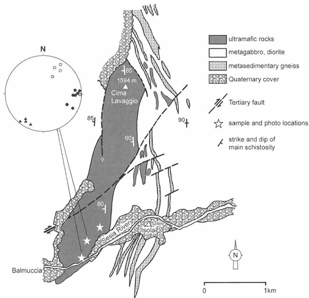
Fig. 2. Geological map of the Balmuccia ultramafic body and surrounding rocks within the Ivrea-Verbano Zone (simplified from Rivalenti et al. 1984; Quick et al. 1994). Equal area projection (lower hemisphere) with poles to foliation of type 1 shear zones (closed triangles) and type 2 shear zones (closed circles) with respect to the average orientation of the pre-existing compositional banding and granulite facies schistosity (open square) in a quarry of the Balmuccia ultramafic complex. Open circles are poles to cracks at the ends of type 2 shear zones.
