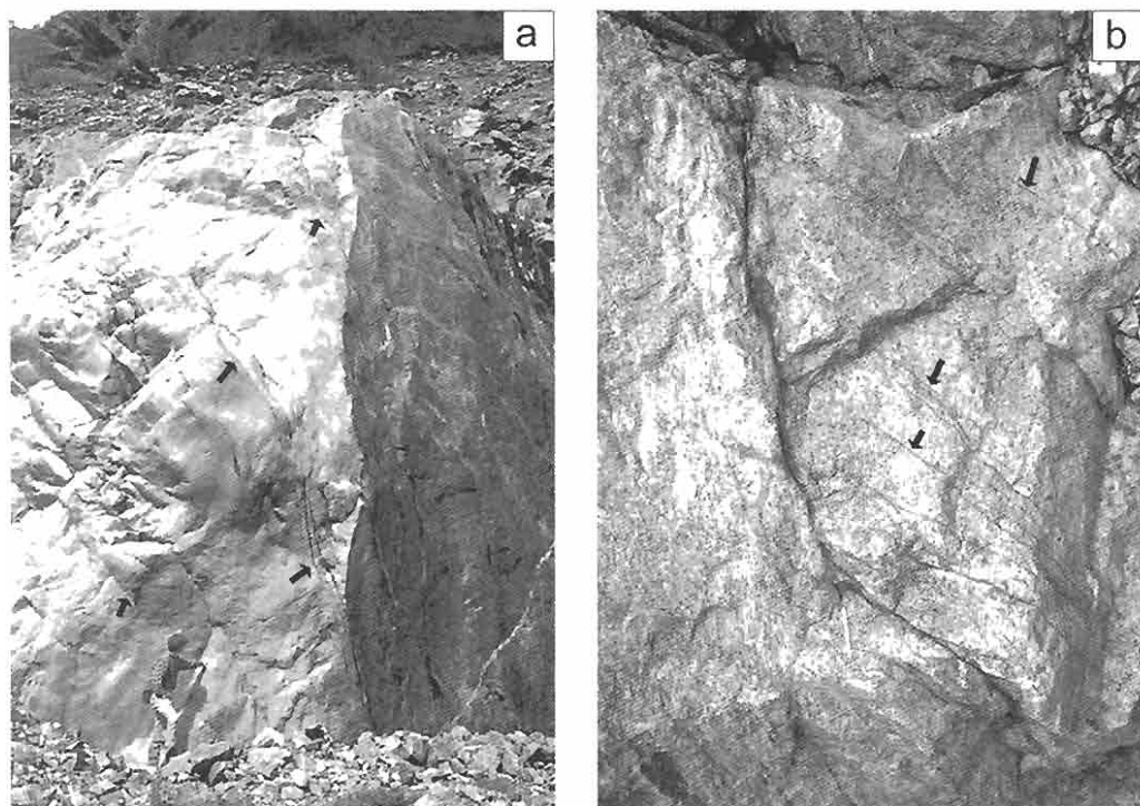
Fig. 3. Shear zones in lherzolite of the Balmuccia ultramafic body. (a) Type 2 shear zones appear as elongate cracks (arrows) and have conjugate orientations. The dark surface to the right is the serpentine-coated surface of such a shear zone. (b) Termination of a type 2 shear zone marked by discordant splays and late pseudotachylite (match tip). Type 1 shear zones (arrows) are truncated by the type 2 shear zone. Match for scale is 5 cm long.
