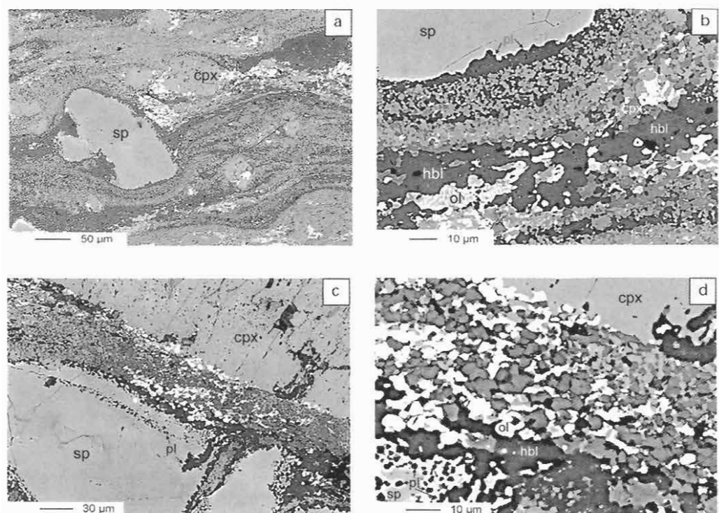
Fig. 6. Backscatter electron (BSE) images of mylonite in a type 1 shear zone. (a) Porphyroclasts of spinel (sp) and clinopyroxene (cpx) embedded in thin laminae of mixed phase layers consisting of olivine, plagioclase, orthopyroxene, clinopyroxene, and hornblende. (b) Detail of (a): boundary of a spinel grain (sp), where plagioclase (dark, pl), clinopyroxene (medium grey, cpx), and hornblende (slightly darker grey, hbl) form. The three new phases are well mixed. (c) A spinel grain (lower left, sp) and a clinopyroxene grain (upper right, cpx). Between these two grains is a thin mixed phase layer of plagioclase (pl), hornblende (hbl), olivine (ol), and clinopyroxene (cpx). (d) Detail of (c), showing the distribution of phases: plagioclase (dark, pl), olivine (lightest grey, ol), hornblende (darker grey, hbl), and clinopyroxene (lighter grey, cpx).
