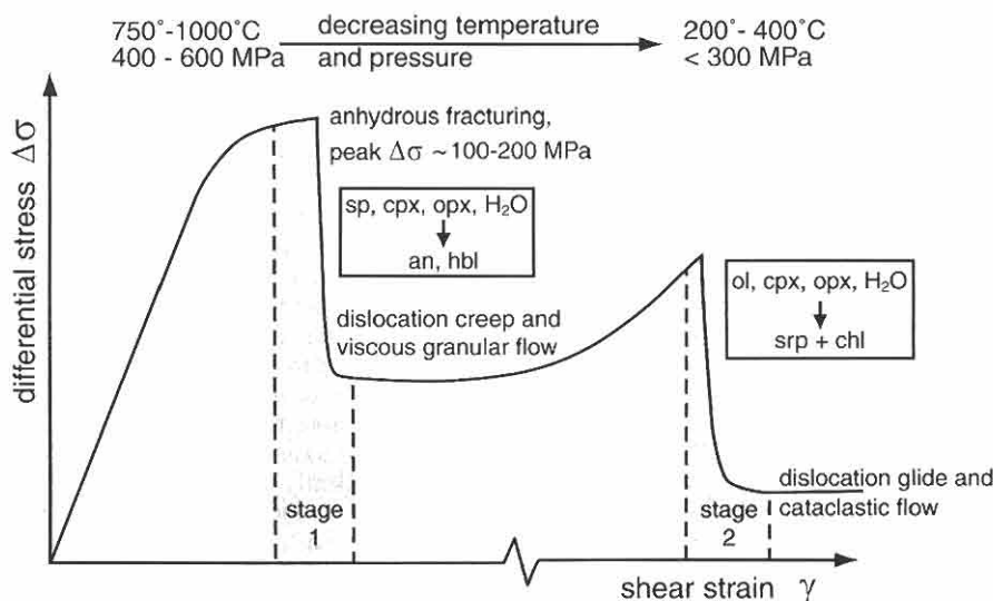
Fig. 10. Schematic strength versus strain evolution of lherzolite in the Balmuccia ultramafic body during Early Mesozoic rifting inferred from microstructures (see text).
