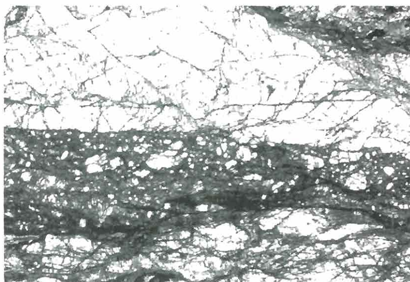
Fig. 8. Cataclastic microstructure of a type 2 shear zone. Note the angular, fractured clasts of partly serpentinized olivine (large clast at top, small clasts in matrix) and a nearly opaque matrix comprising mainly ultrafine grained serpentine and chlorite. View in the XZ fabric plane. Length of micrograph is 3.4 mm.
