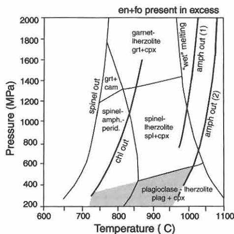
Fig. 9. P-T diagram for ultramafic rocks with the inferred pressure and temperature fields for the high-temperature shear deformation during Early Mesozoic rifting of the upper mantle. Stability fields and curves for stability of spinel and chlorite after Bucher & Frey (1994), experimentally determined hornblende stability curves from Wallace & Green (1991) (amph-out, 1) and Niida & Green (1999), (amph-out, 2). The probable maximum pressure and temperature range for the high temperature deformation of type 1 shear zones is indicated by grey shading.
