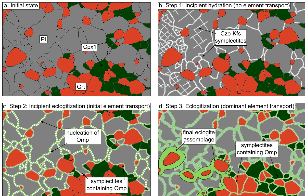
Fig. 8 Sketch of the initial granulite and the changes associated with each step of the reaction. a Initial granulite microstructure. b Incipient hydration with symplectites of Zo/Czo-Kfs + albite Pl along Pl–Pl grain boundaries and later throughout the Pl grains. For simplicity, the Zo/Czo-Kfs symplectites within the grains are only shown in b , where they form and are omitted in the following images. c Incipi-
